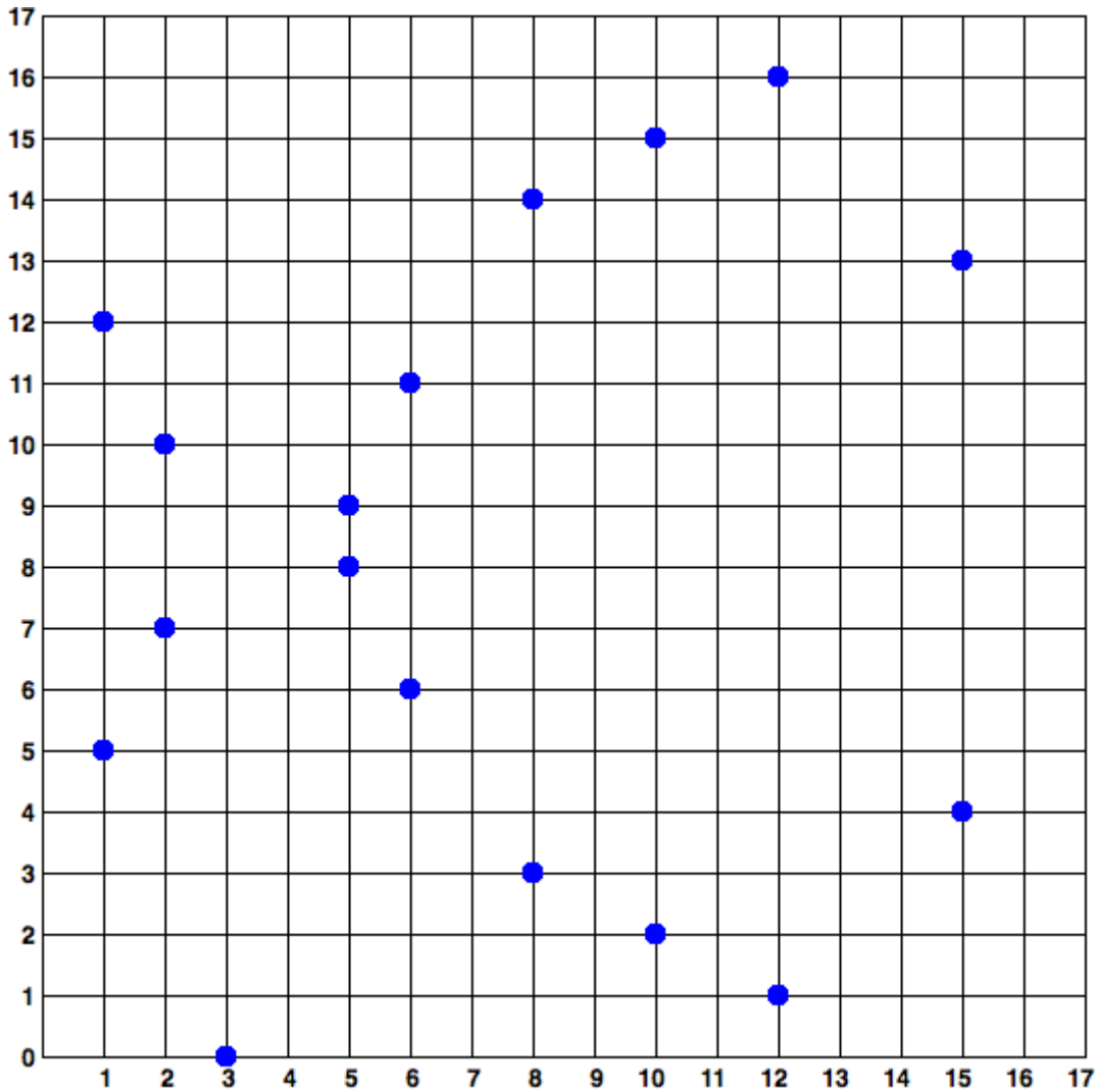
Figure 19. Elliptic curve cryptography: visualizing an elliptic curve over F(p) , with p=17
