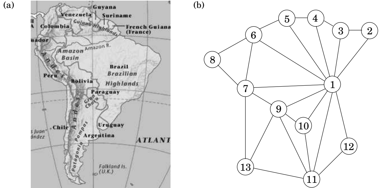
Figure 3.1 (a) A map and (b) its graph.
